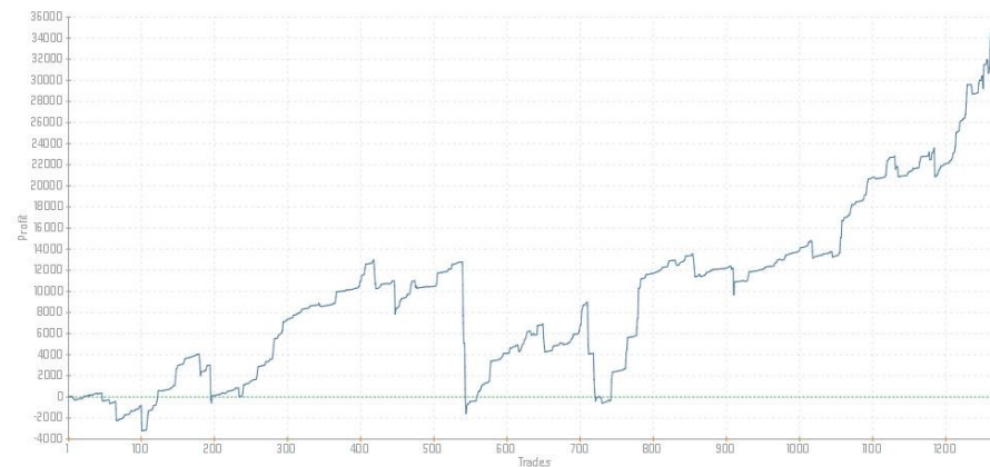
Summary Stats
